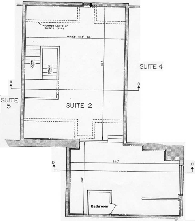
Second Floor
